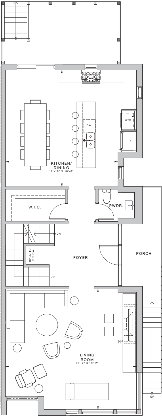
MAIN FLOOR 1,176 SQ.FT.
