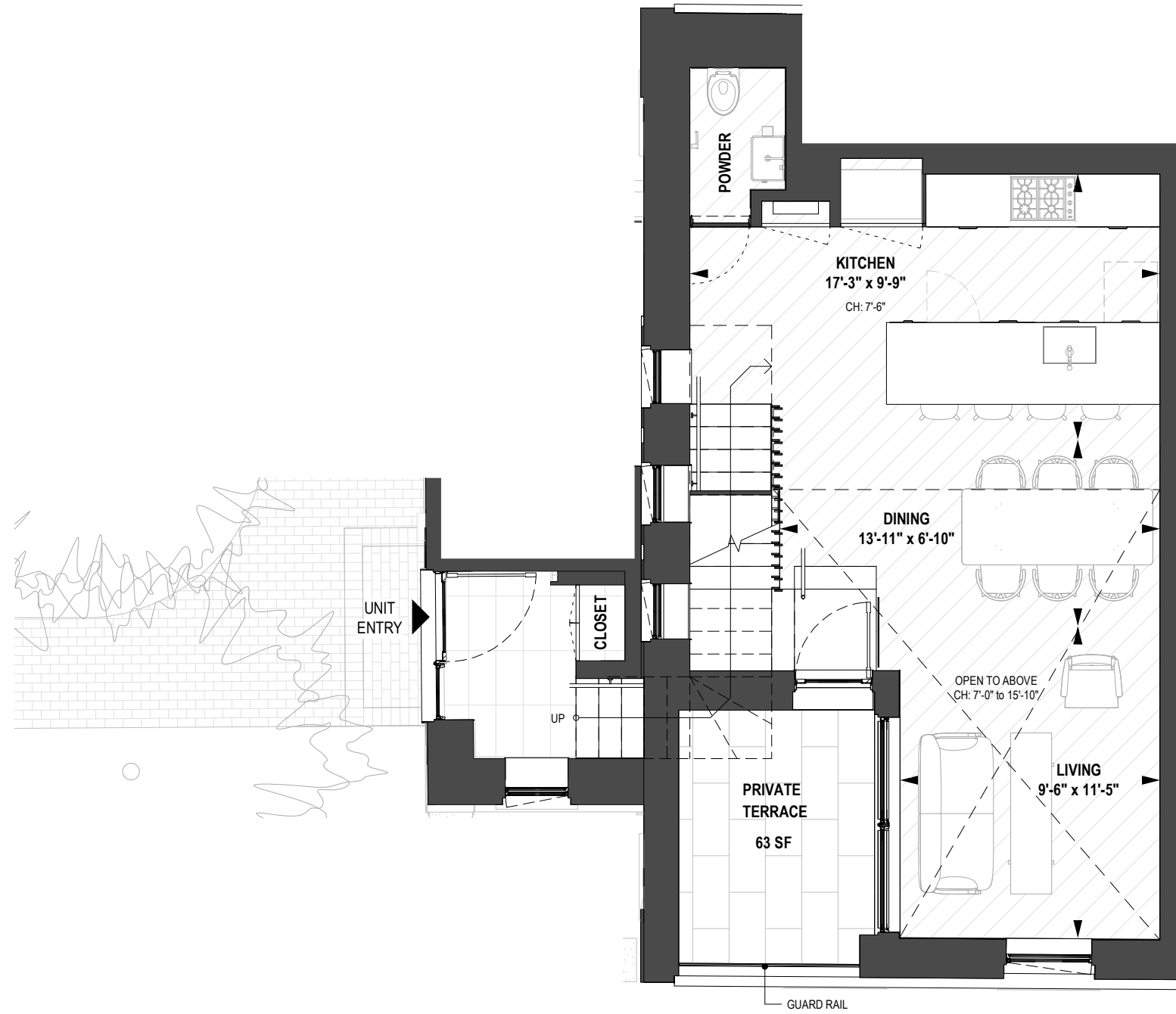
UNIT 2 ENTRY & LOWER LEVEL 1 1 : 64
