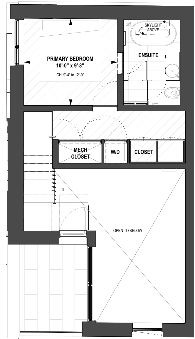
UNIT 2 UPPER LEVEL 2 1 : 64
