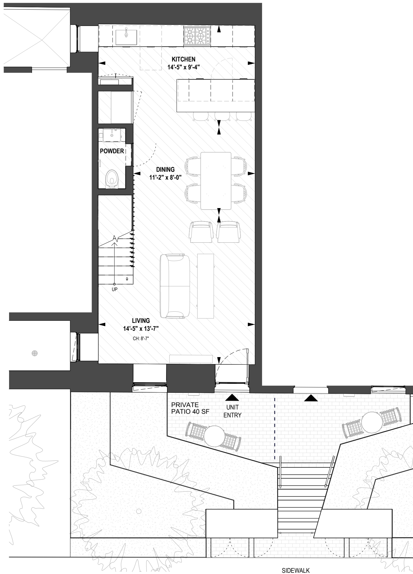
UNIT 3 LOWER LEVEL 1 1:64
