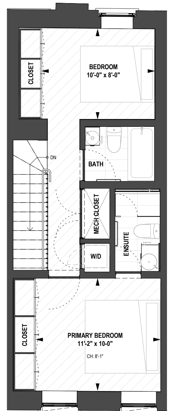
UNIT 4 UPPER LEVEL 2 1:64
