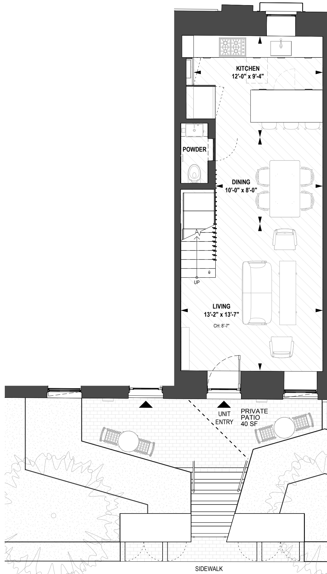
UNIT 4 LOWER LEVEL 1 1:64
