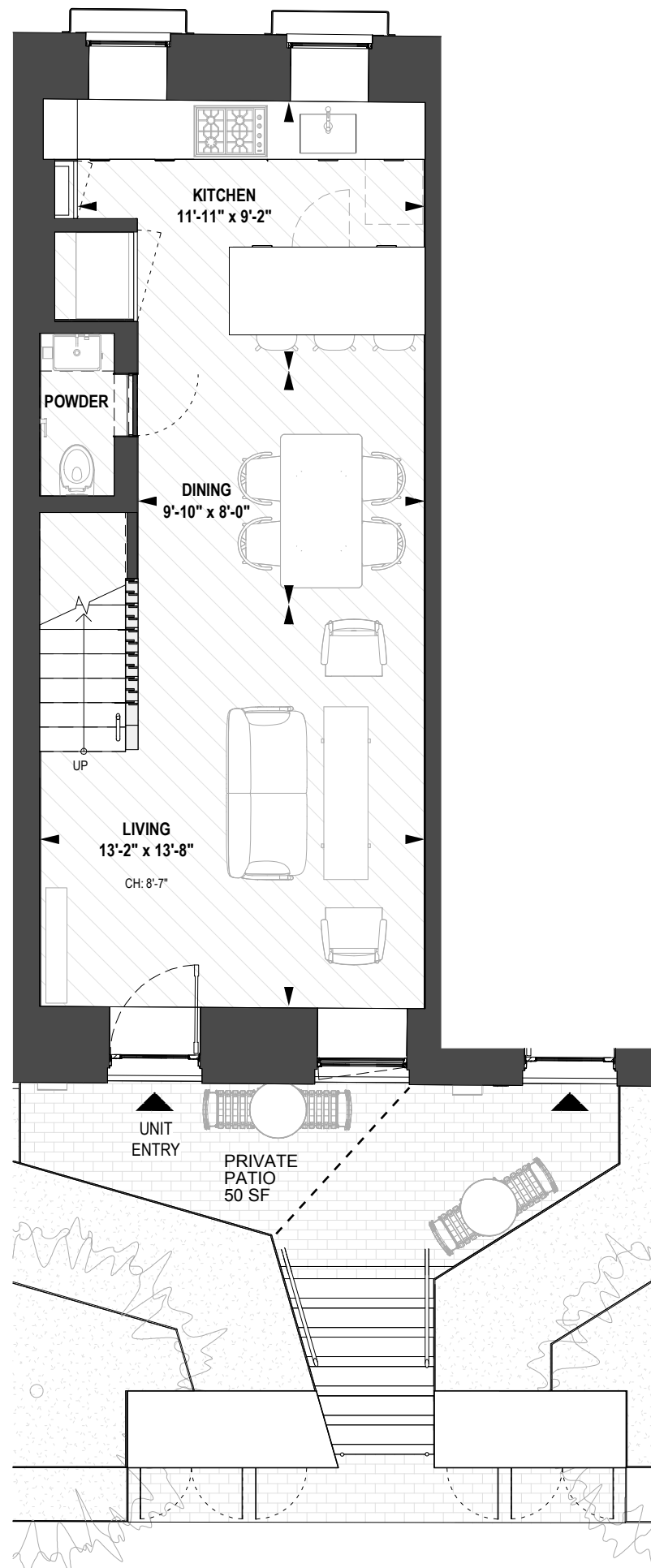
UNIT 5 LOWER LEVEL 1 1:64
