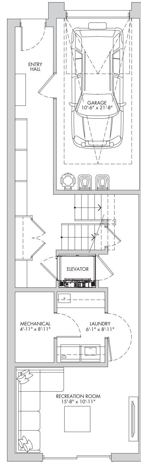
LOWER LEVEL. 746 SQ.FT.
