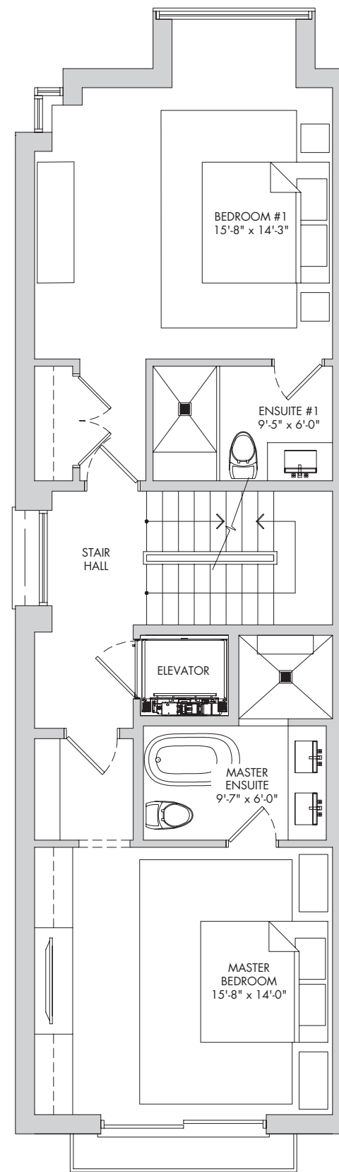
SECOND FLOOR. 982 SQ.FT.
